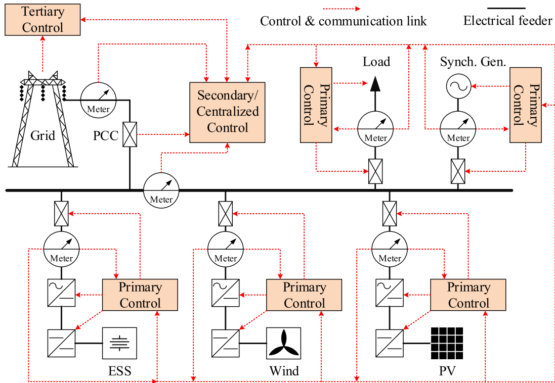
Fig. 1. Typical configuration of a microgrid.
