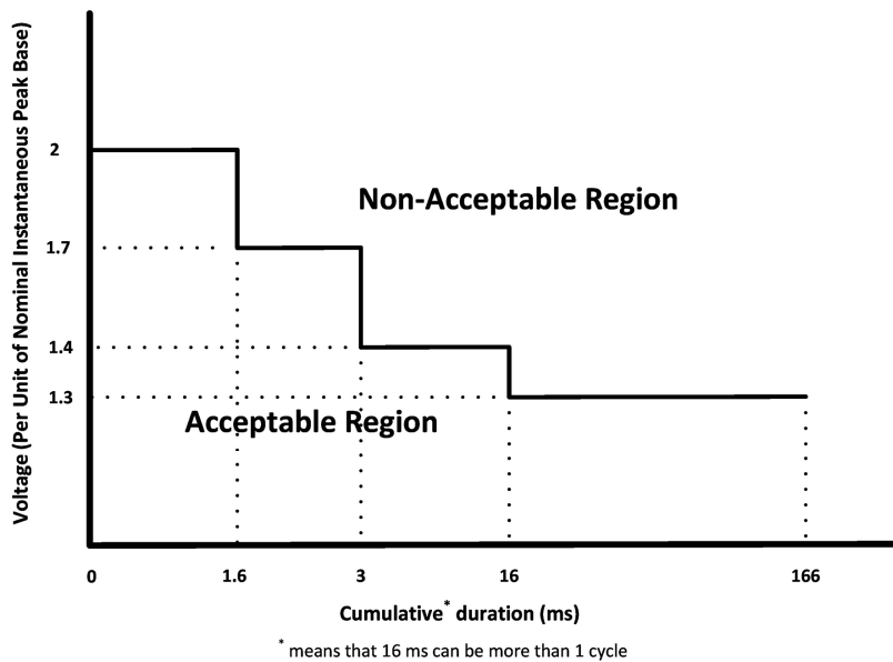
Figure 3 —Transient overvoltage limits
